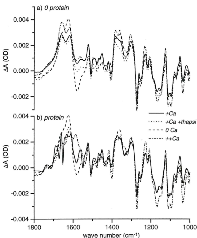
FIGURE 3 IR spectra induced by post-photolytic reactions of the DM-nitrophen photoproduct. Kinetic measurements were performed on medium and protein samples as described in Materials and Methods and in Scheme 2. The temperature was -8.8 \pm 0.4^\circ\text{C} . The spectra shown on the figure are averaged over the time period between 923 and 1255 s after the flash for four to eight medium samples (a) and protein samples (b), as all reactions are completed. The indications on the figure refer to the different measuring conditions, which are described in Materials and Methods. Similar bands induced by reactions of the DM-N photoproduct arise in all conditions over the 1750\text{--}1000\text{ cm}^{-1} range, in the absence and presence of SR vesicles.
