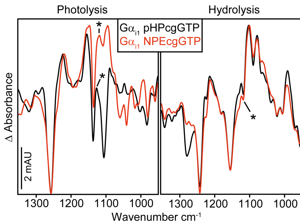
Supplemental Figure 10: FTIR difference spectra of G\alpha_{i1} -WT with pHPcgGTP and NPEcgGTP. The band at 1120\text{ cm}^{-1} (*) is assumed to be the second asymmetrical \gamma -GTP band.
