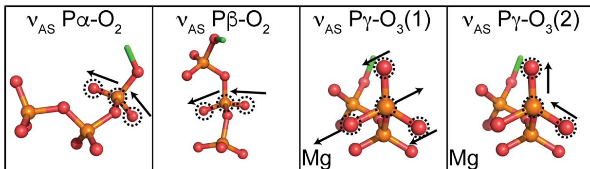
Supplemental Figure 5: Schematic displacement vectors of the calculated GDP infrared frequencies
