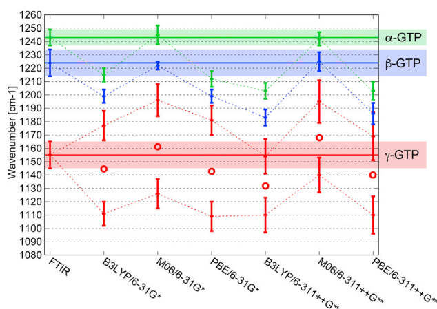
FIGURE 3 Calculated IR spectra of GTP bound to G\alpha_{i1} with different levels of theory in comparison with experimental values (FTIR). Standard deviations (bars) are also depicted and compared with the FWHM values of the experiments. Mean values of the \gamma -GTP vibration are indicated by dots to enable comparison of band shifts with the experiments that will be discussed below. To see this figure in color, go online.
