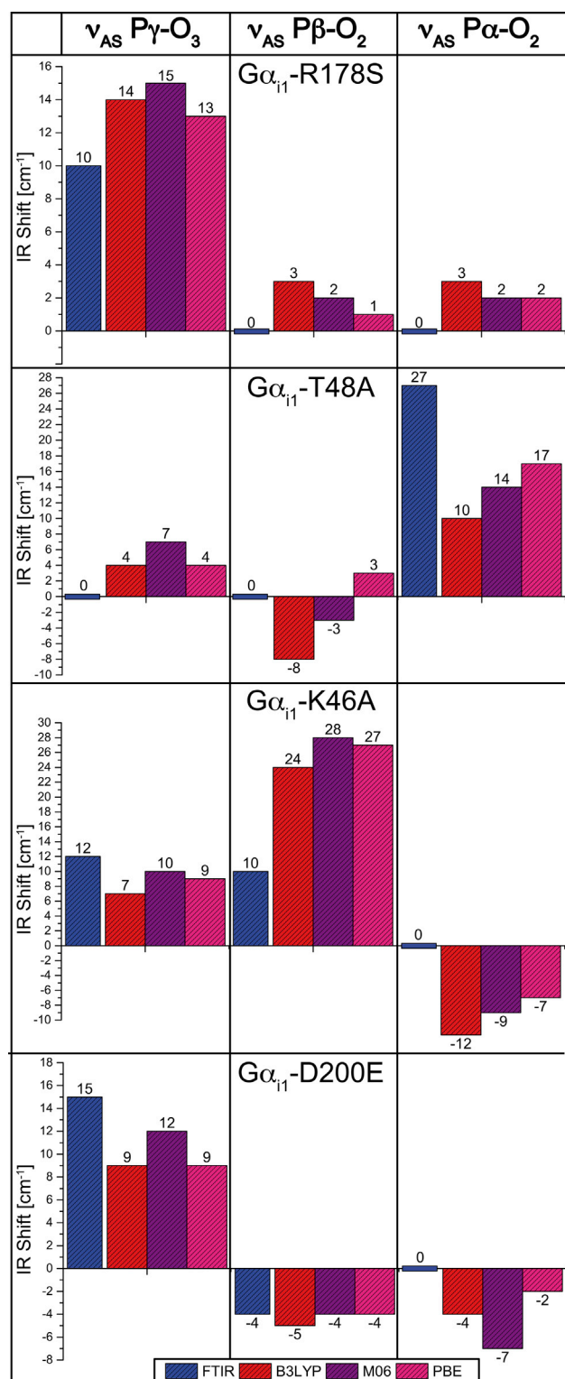
FIGURE 6 Calculated infrared absorption band shifts of G\alpha_{i1} point mutants with respect to wild-type simulations. Experimental shifts are depicted in blue and calculated shifts are depicted in red shades for each individual phosphate group. To see this figure in color, go online.
