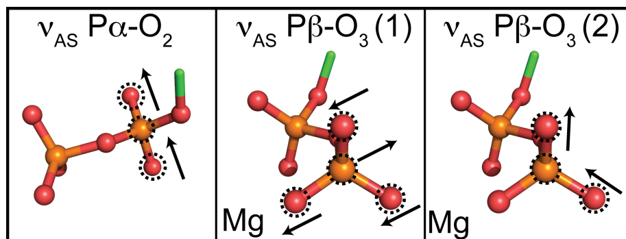
Supplemental Figure 5: Schematic displacement vectors of the calculated GDP infrared frequencies
